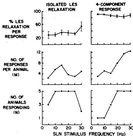
Figure 2. Comparison of two response types, namely, isolated LES relaxation and full four-component swallowing sequence with respect to three variables: (a) number of animals responding ( N ) out of a total of five; (b) mean number of responses per responding animal ( M ); and (c) mean percent LES relaxation per response (mean of means in each animal \pm SE). For the isolated LES relaxation response, N and M tend to be lowest at the high and low extremes of SLN stimulus frequency and highest at the mid-range of frequencies, whereas for the full four-component response N and M increase with increasing stimulus frequency. The mean percent LES relaxation is significantly lower for the isolated LES relaxation response than for the full four-component response at all SLN stimulus frequencies tested ( P < 0.05 at 30 Hz and P < 0.001 at 5, 10, 15, 20, and 25 Hz). There is no statistically significant difference between the magnitude of LES relaxation at the different SLN stimulus frequencies for the full four-component type response. For the isolated LES relaxation response, the magnitude of LES relaxation at 5 and 10 Hz was significantly less than that at 30 Hz ( P < 0.05 ).
