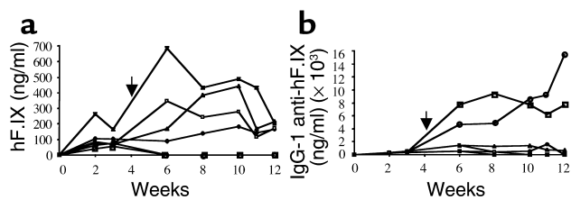
Figure 6 Liver-directed gene transfer with AAV-EF1 \alpha -hF.IX vector ( 2 \times 10^{11} vg/animal) in C57BL/6 mice deficient in cell death receptor Fas ( n = 6 ). Shown are plasma levels of hF.IX and anti-hF.IX (measured by ELISA or immuno-capture assay) as a function of time after vector administration. (a) Plasma levels of hF.IX (ng/ml). (b) IgG1 anti-hF.IX. Vertical arrows indicate challenge by subcutaneous administration of 2 \mu g hF.IX formulated in CFA. Symbols are identical for hF.IX and anti-hF.IX levels of the same animal.
